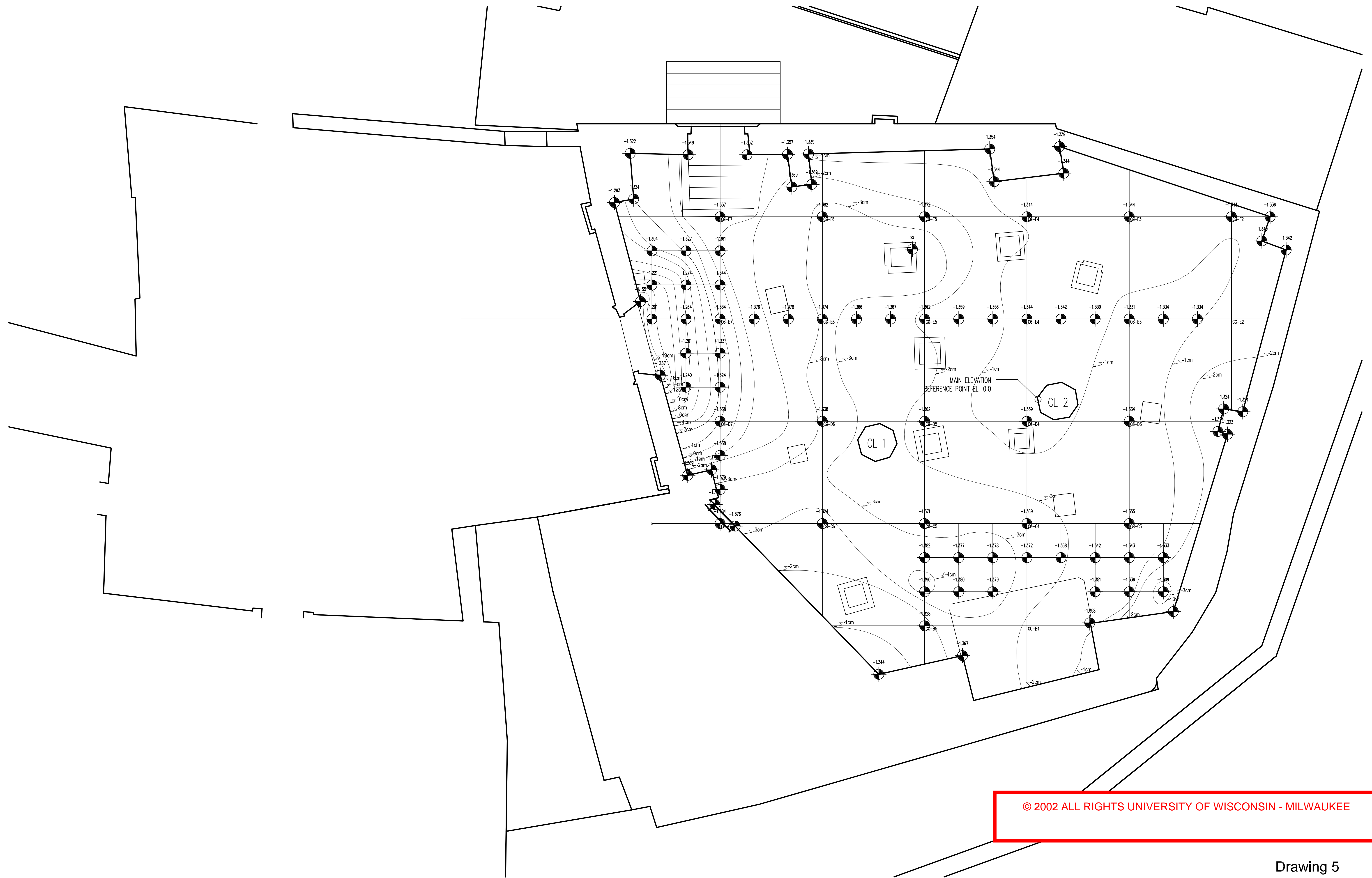
CHURCH FLOOR TOPOGRAPHY - 1 & 2 Cm . Contours Scale 1:50
