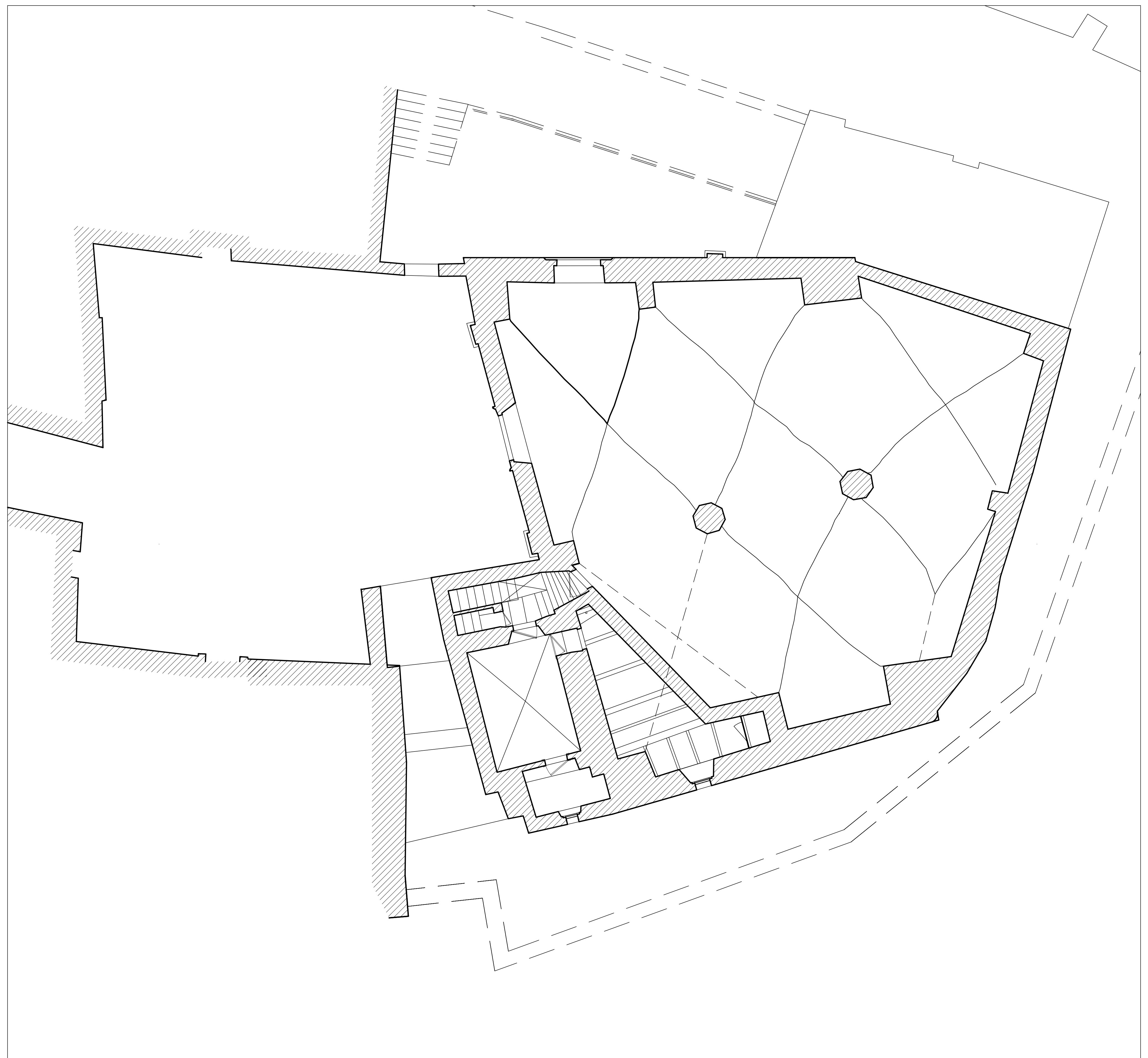
Ground Level Reflected Ceiling Plan - Church & Courtyard
